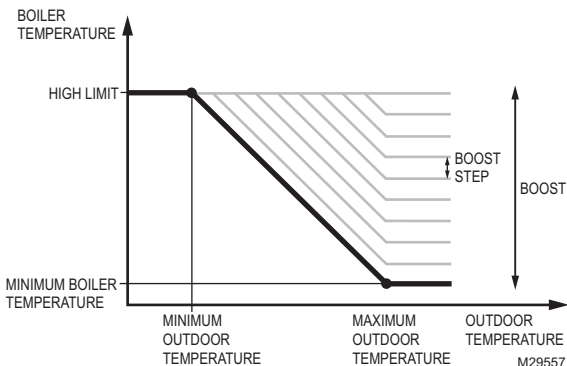
Fig. 1. Outdoor temperature setback curve with boost.
